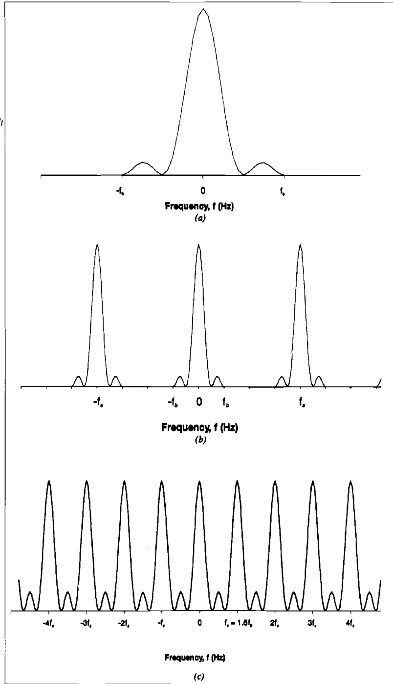
2. (a) A hypothetical FT, X_1(f) , for discussion purposes. Note that X_1(f) is generally a complex function of f , which can therefore only be correctly drawn in three dimensions. However, since x_1(t) is real and even, the FT X_1(f) happens to be real and even in this case. (b) The periodic FT Y(f) when f_s > 2f_b . (c) The periodic FT Y(f) when f_s \leq 2f_b .
