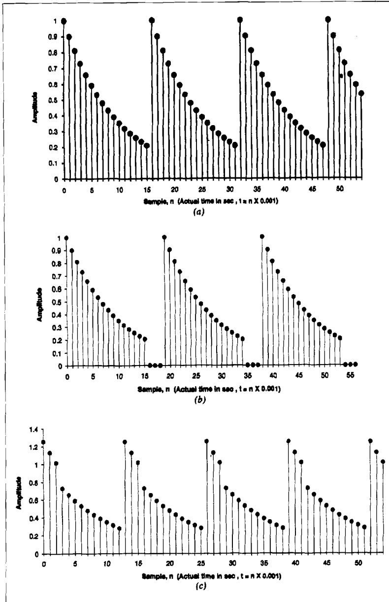
7. The signal y(nT_s) of Eq. 24 when (a) f_y = 1/NT_s = f_s/N ; (b) f_y < 1/NT_s ; (c) f_y \geq 1/NT_s . Each waveform repeats indefinitely in both positive and negative time.
